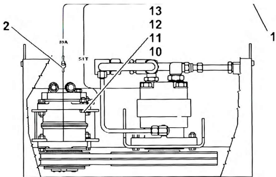
VIEW A TOP VIEW OF AC COMPRESSOR AND MOTOR ASSEMBLY (SCALE 1:2)
