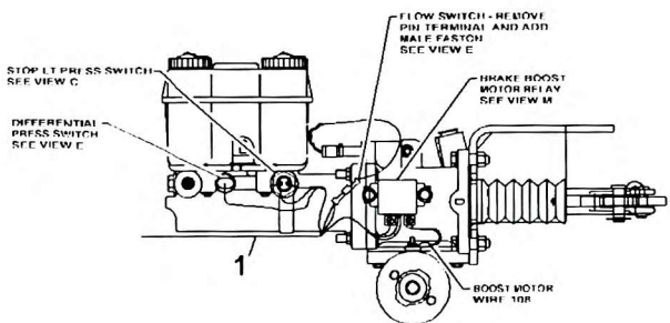
VIEW B BRAKE BOOST
